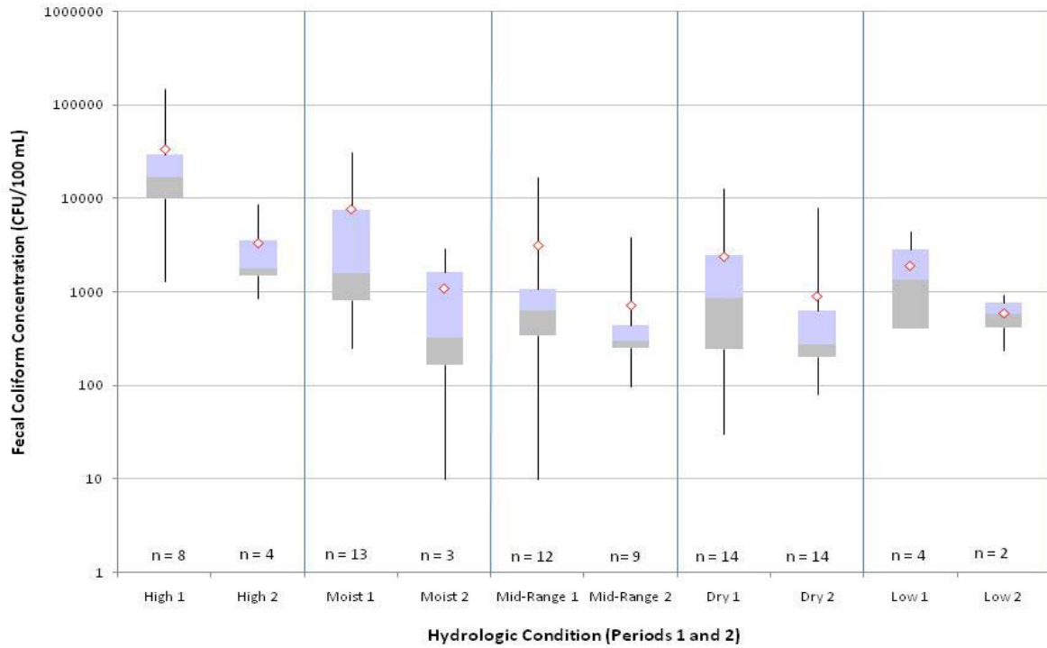
Figure 16. Oostanaula Creek TMDL implementation effectiveness (box and whisker plot).
