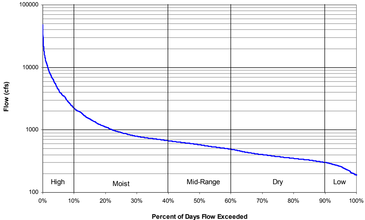
Figure 14. Five-Zone Flow Duration Curve for Wolf River at RM 1.5.
