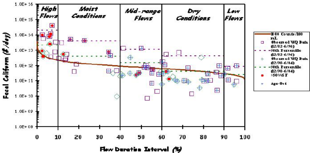
Figure 17. Oostanaula Creek TMDL implementation effectiveness (LDC analysis).
