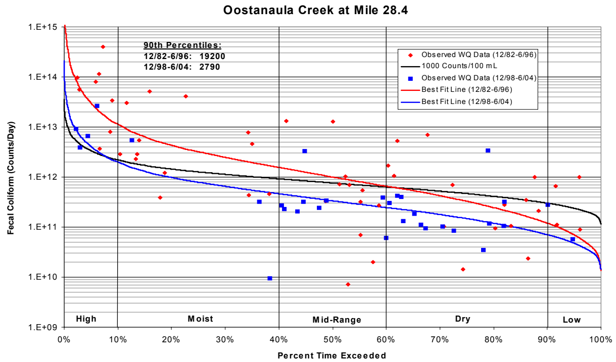
Figure 18. Oostanaula Creek TMDL implementation effectiveness (LDC regression analysis).
