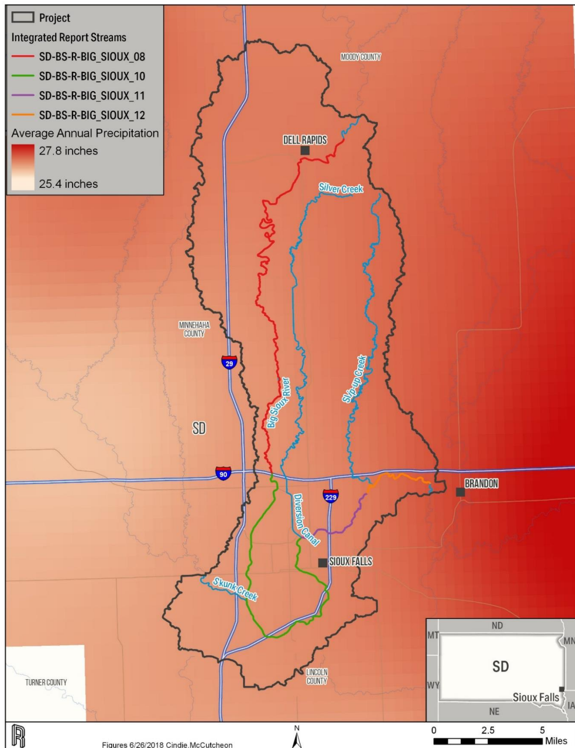
Figure 1-2. PRISM Average Annual Precipitation From 1981 to 2010.
