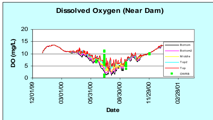
FIGURE 6-24. DISSOLVED OXYGEN NEAR THE DAM (2000)
