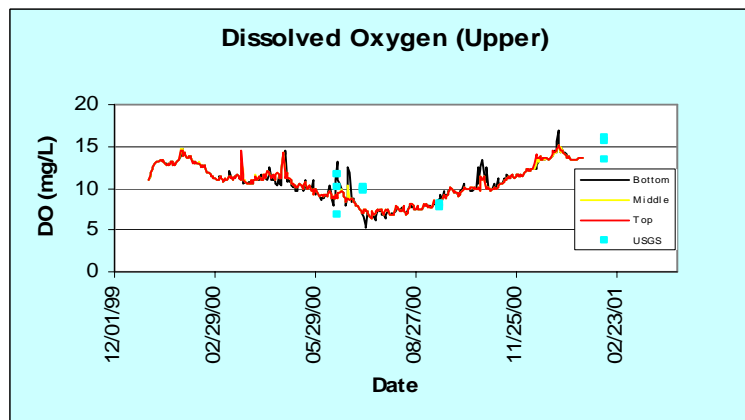
FIGURE 6-26. DISSOLVED OXYGEN IN THE UPPER PART OF THE LAKE (2000)
