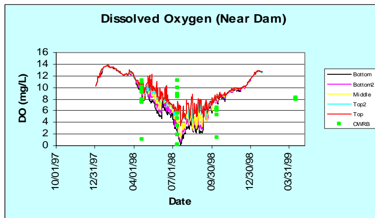
FIGURE 6-10. DISSOLVED OXYGEN NEAR THE DAM
