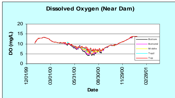
FIGURE 7-7. DISSOLVED OXYGEN NEAR THE DAM (REDUCTION)
