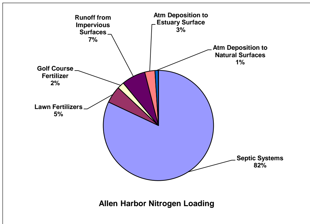
Figure ES-A: Percent Contributions of All Nitrogen Sources to Allen Harbor Embayment System
