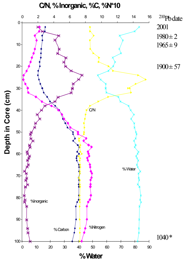
Figure 1. Elemental composition of core. Nitrogen values are magnified by one order of magnitude in order to show trends. 210 Pb dates are shown \pm one standard deviation. *extrapolated date based on a sedimentation rate of 0.93mm per year from lowermost 210 Pb dated sections of the core.
