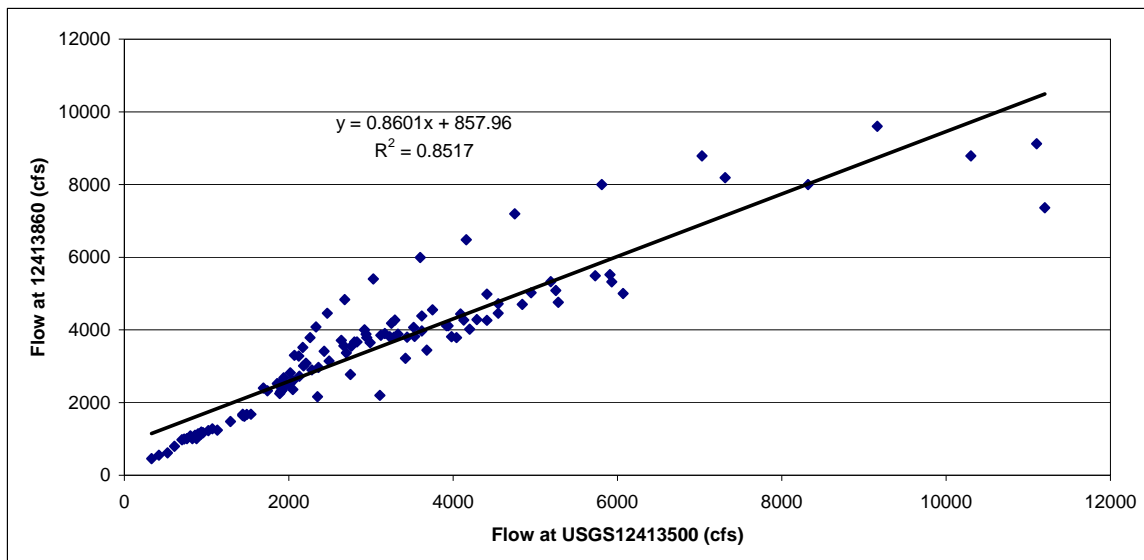
Figure C-1. Flow Regression between Cataldo and Harrison USGS Gages
