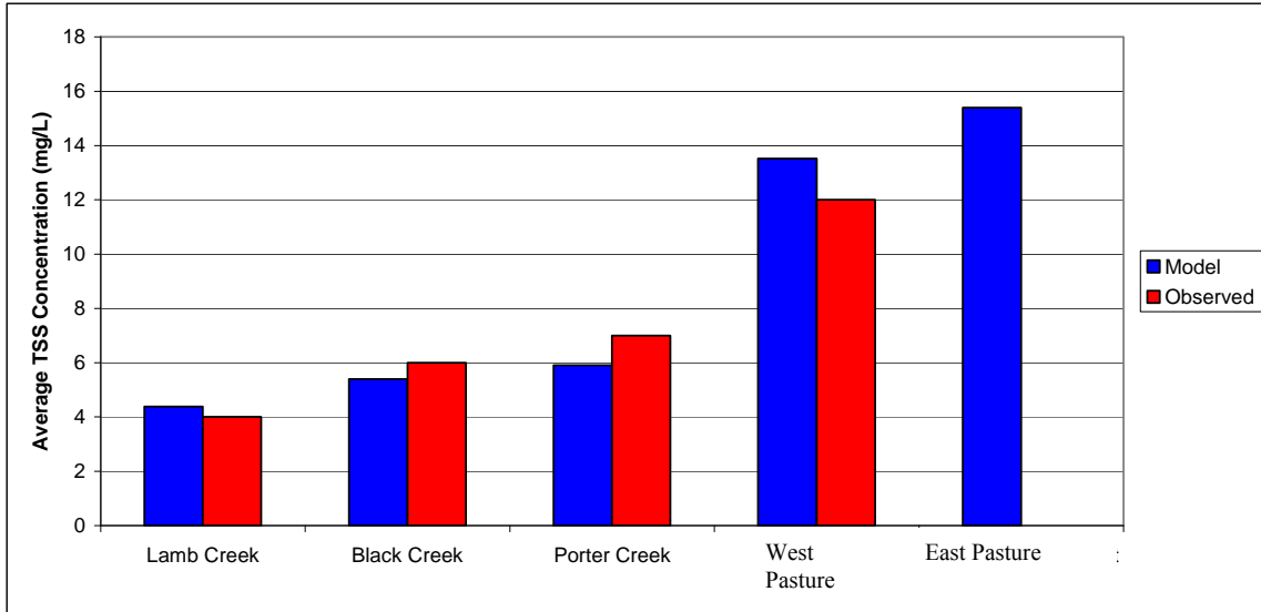
Figure F-2. Observed and Modeled Average TSS Concentrations
