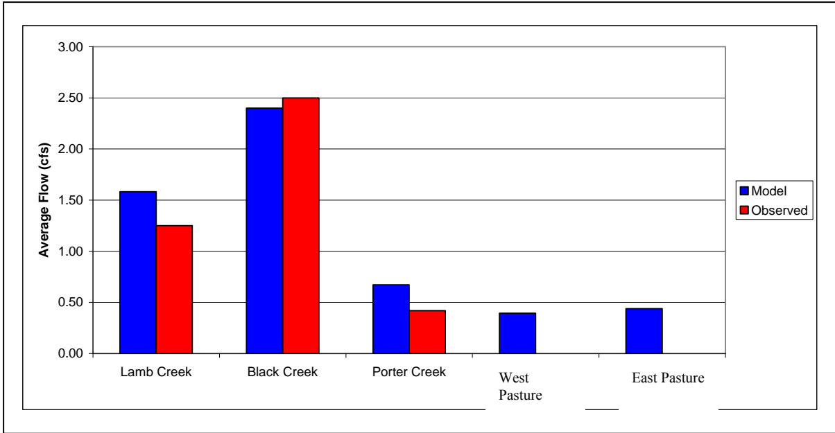
Figure F-1. Observed and Modeled Annual Average Flows
