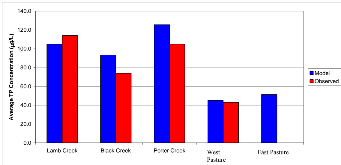
Figure F-3. Modeled and Observed TP Concentrations
