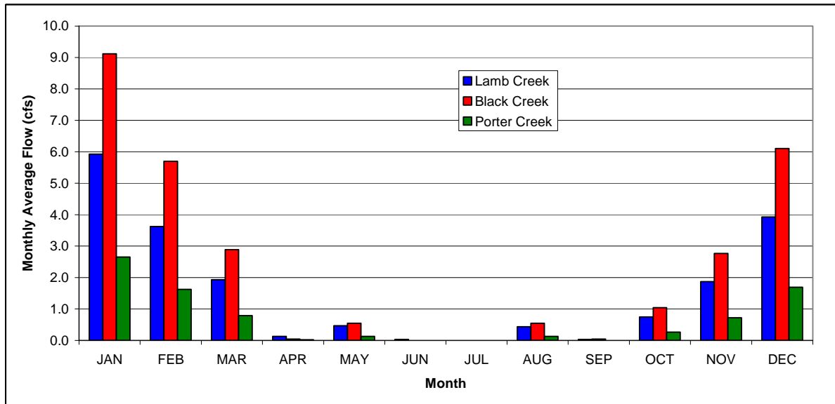
Figure 6. Six-year Average Annual Hydrographs for Black Lake Tributaries
