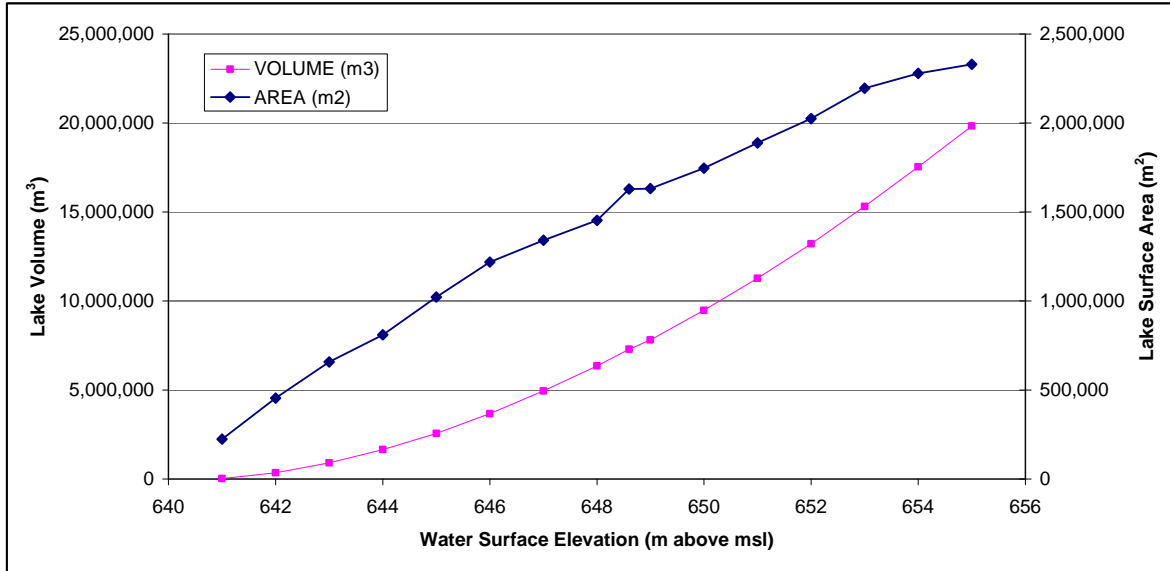
Figure C-3. Rating Curves for Black Lake
