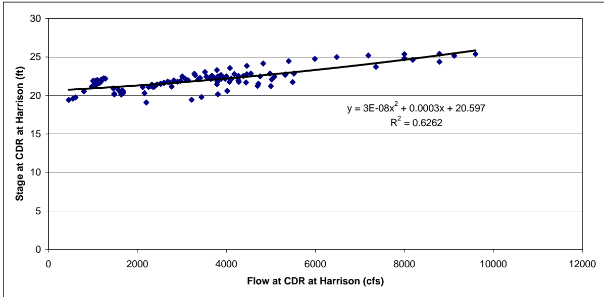
Figure C-2. Rating Curve for the USGS Gage in CDR at Harrison
