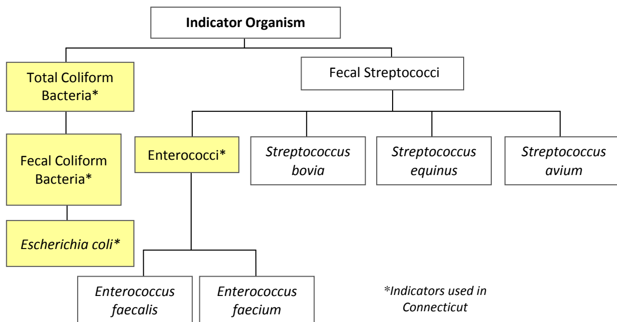
Figure 2-1: Relationship among Indicator Organisms (USEPA, 2001).
