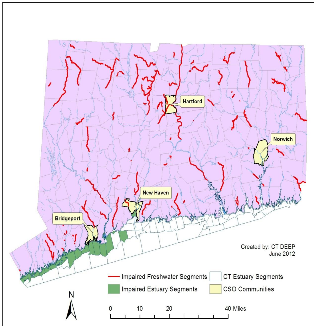
Figure 2-2: CSO Communities in Connecticut. The impairments displayed in this map do not include any segments provided in Appendix A.
