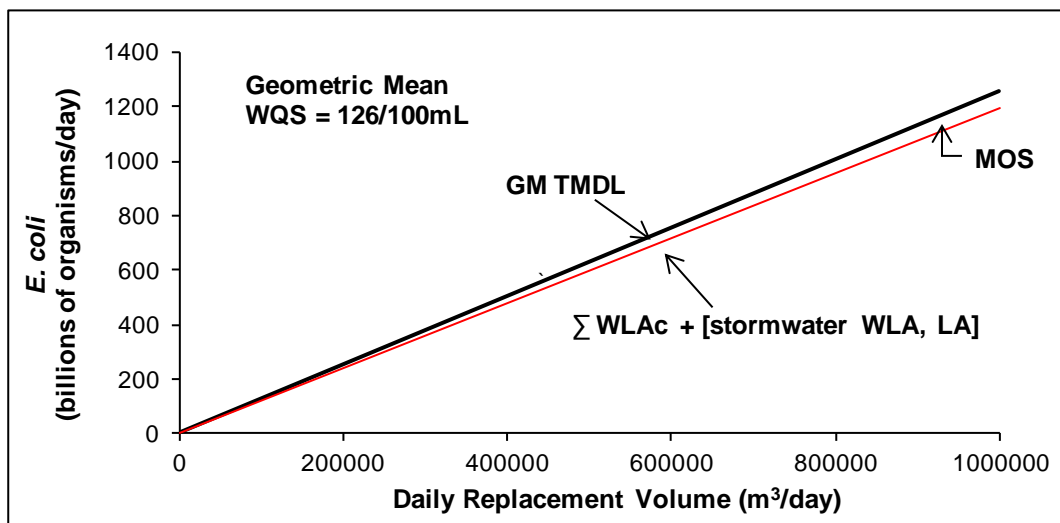
Figure 2: Freshwater lakes and ponds daily loads based on E. coli geometric mean water quality standards (GM WQS).
