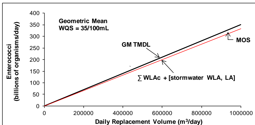
Figure 3: Estuarine and marine daily loads based on Enterococci salt water geometric mean water quality standards (GM WQS).
