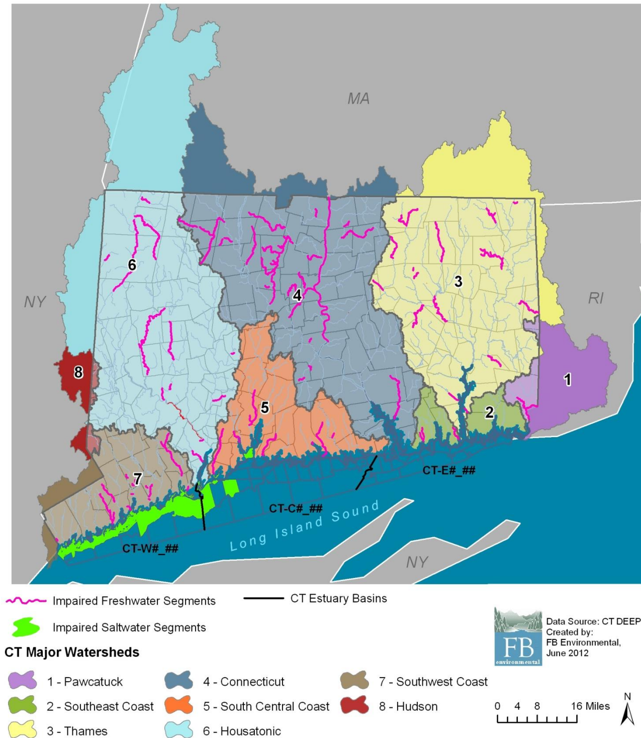
Figure 4-1: Bacteria-Impaired Waterbodies Included in Initial TMDL and Major Watersheds in Connecticut.
