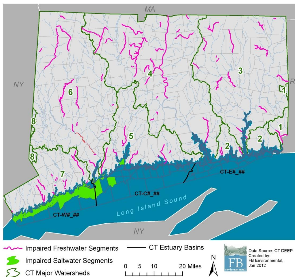
Figure 8-1: Bacteria-Impaired Waters in Connecticut, by Major Watershed and Long Island Sound Division.
