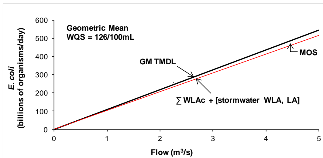
Figure 1: Freshwater rivers and streams daily load based on E. coli geometric mean water quality standard (GM WQS).
