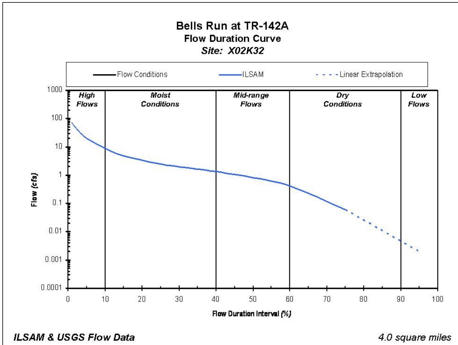
Figure C-7. Flow duration curve for station X02K32.
