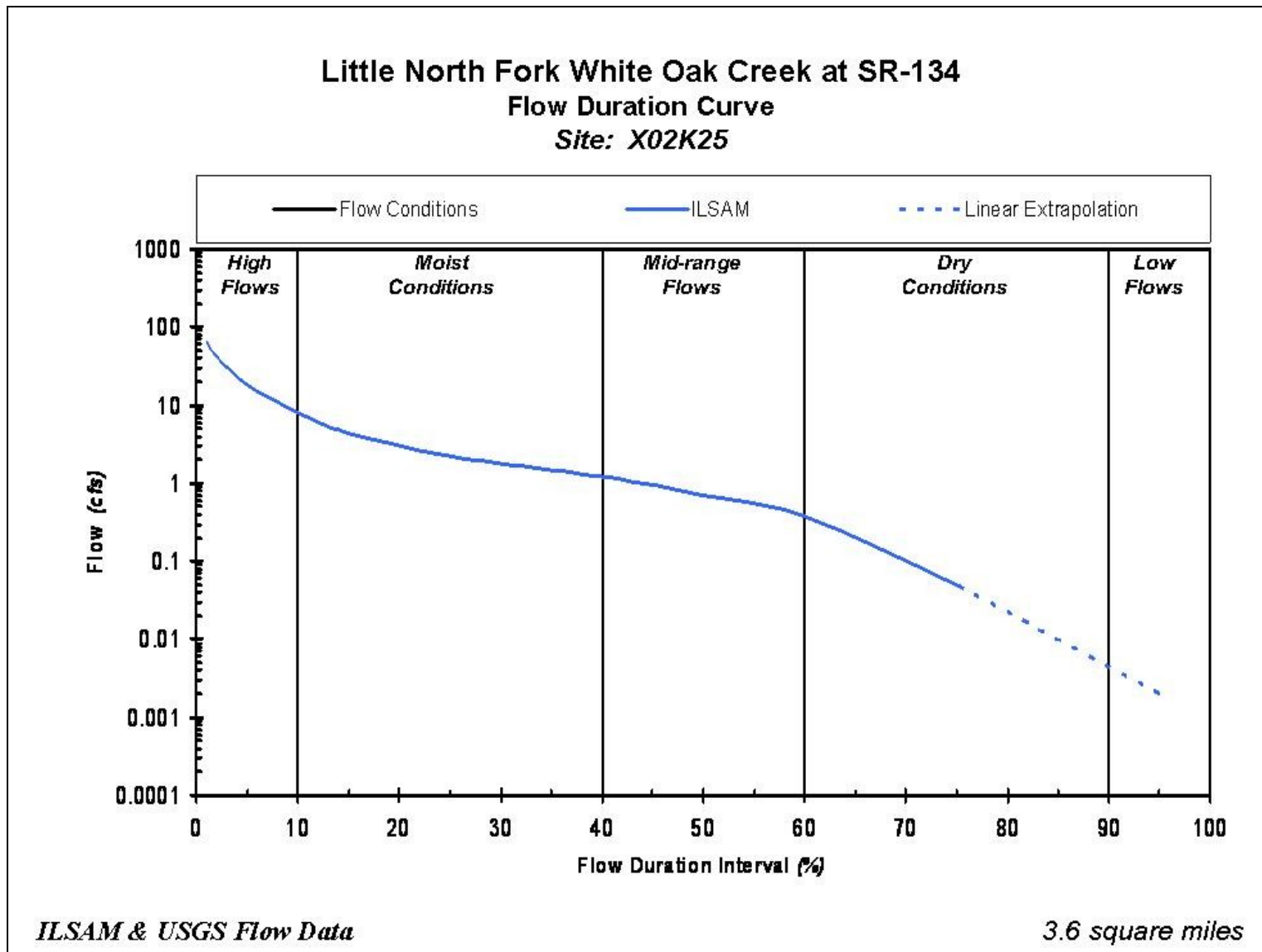
Figure C-4. Flow duration curve for station X02K25.
