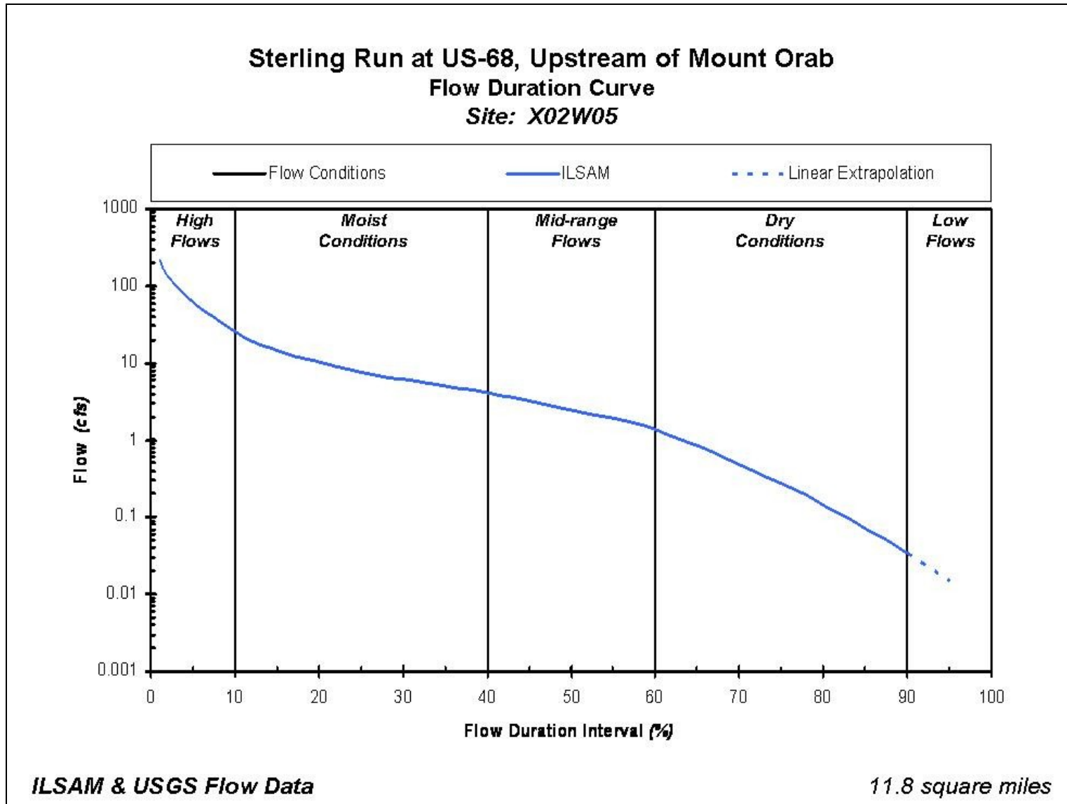
Figure C-9. Flow duration curve for station X02W05.
