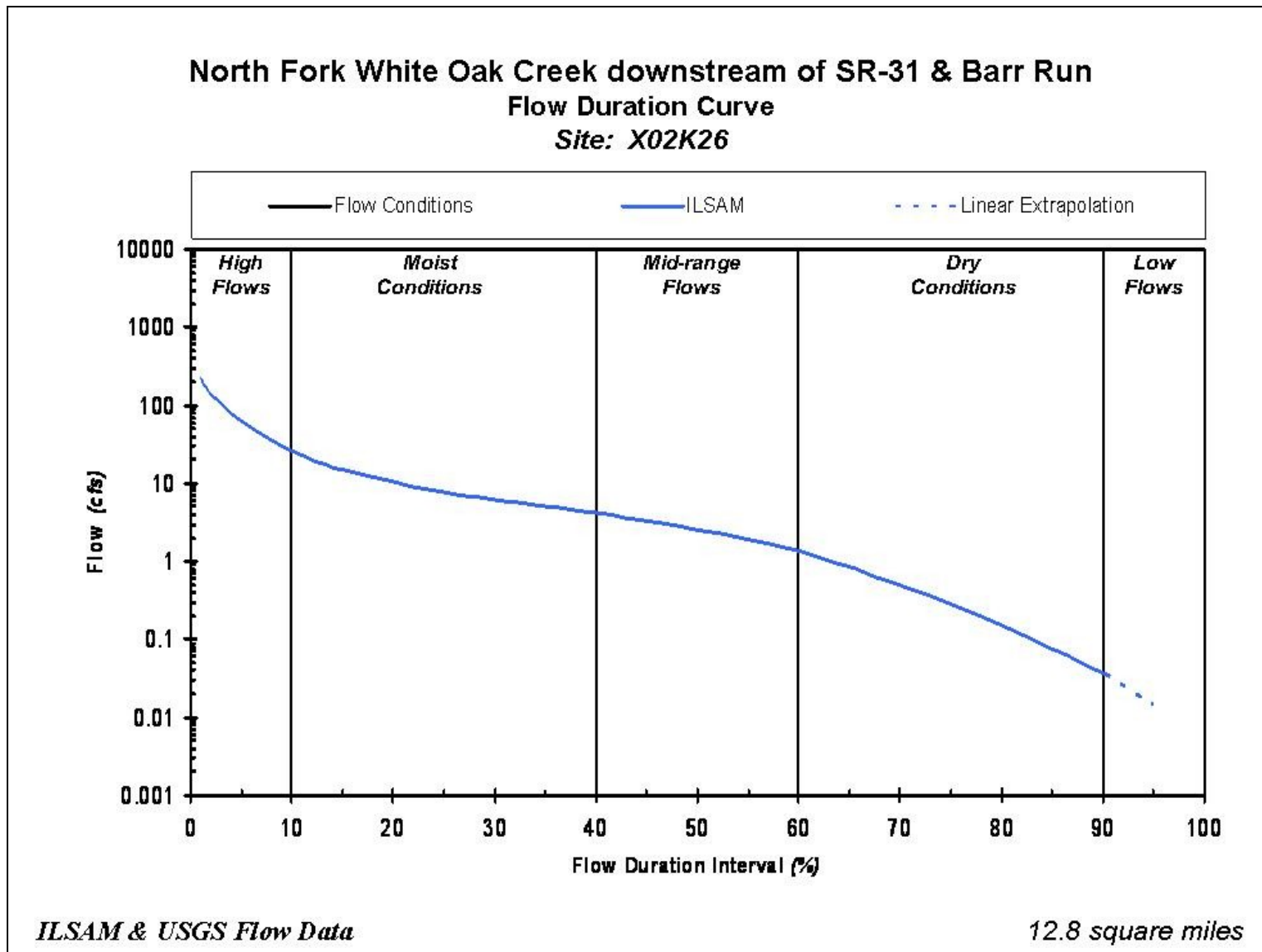
Figure C-5. Flow duration curve for station X02K26.
