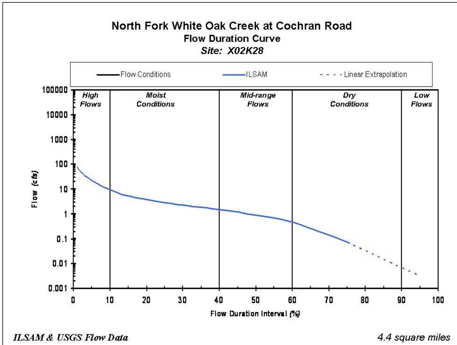
Figure C-6. Flow duration curve for station X02K28.
