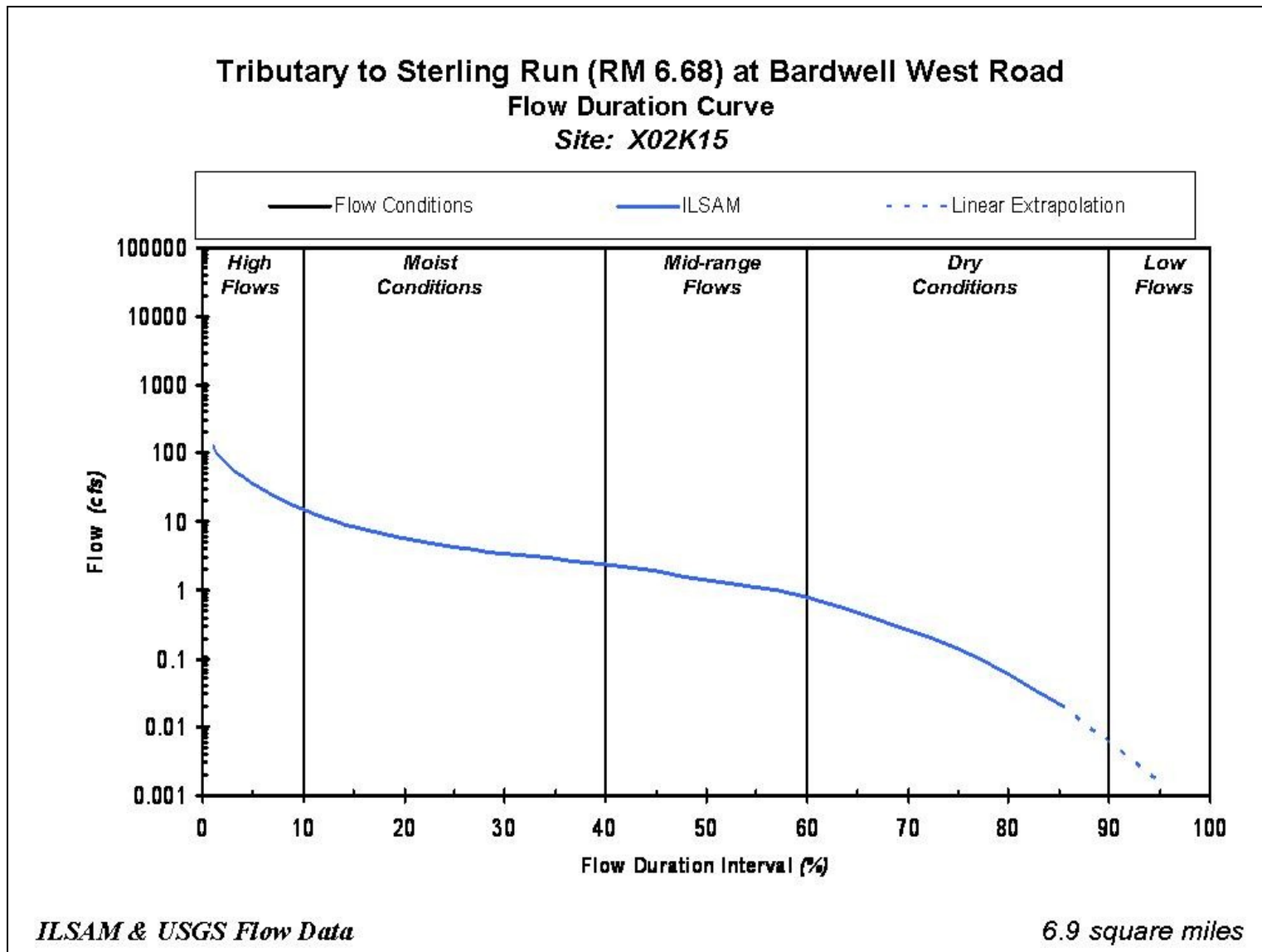
Figure C-1. Flow duration curve for station X02K15.
