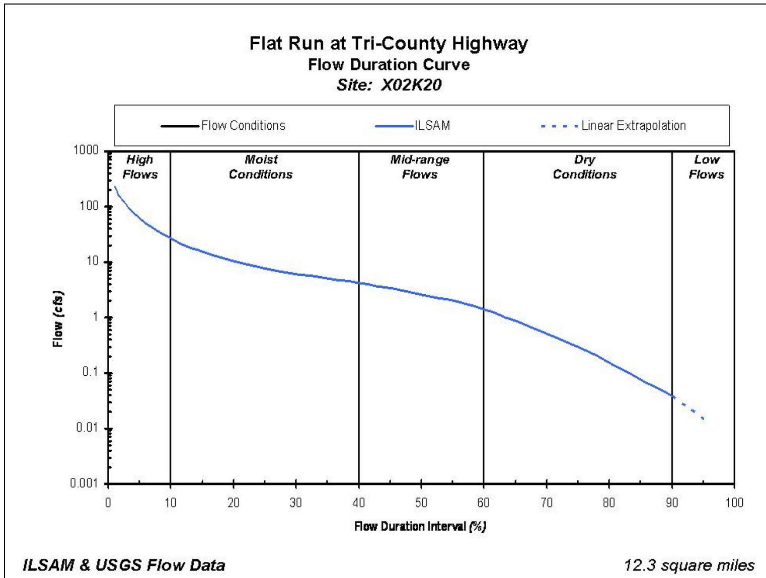
Figure C-3. Flow duration curve for station X02K20.
