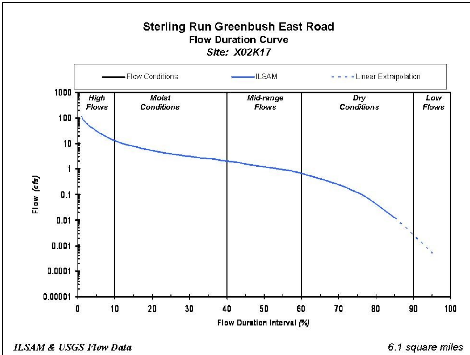
Figure C-2. Flow duration curve for station X02K17.
