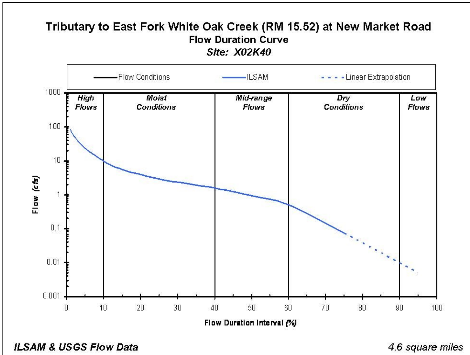
Figure C-8. Flow duration curve for station X02K40.
