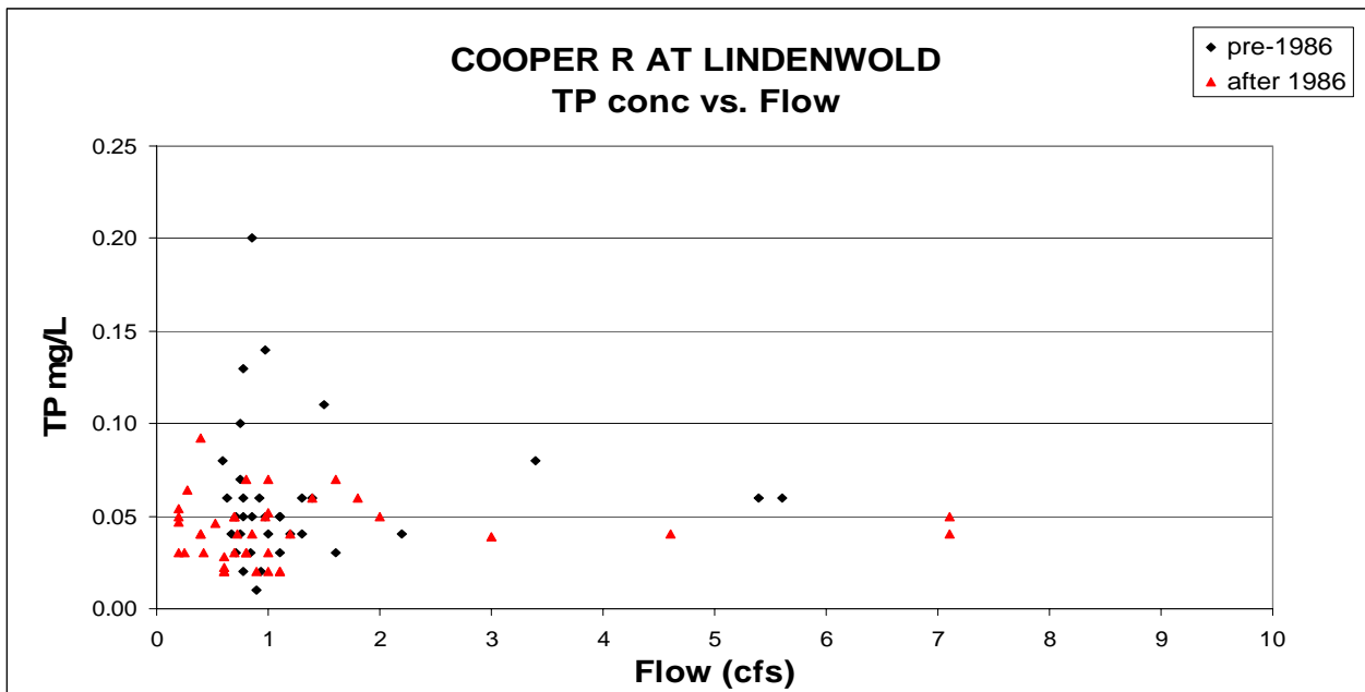
Figure 6 Changes in Phosphorus Concentration with Flow
