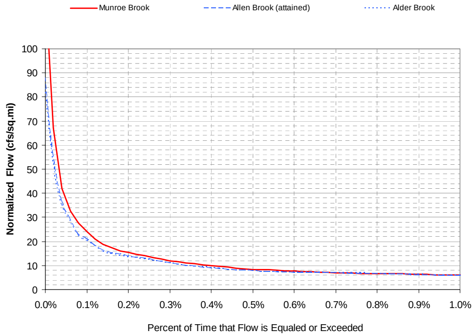
Figure 5. High flow portion of the flow duration curves for Munroe Brook and attainment streams
