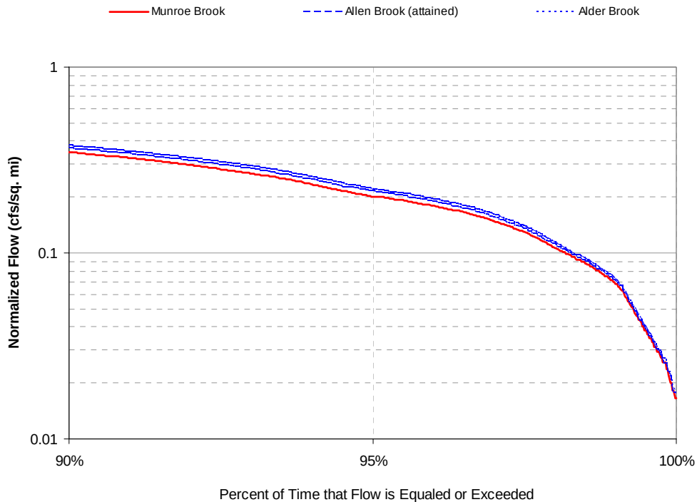
Figure 6. Low flow portion of the flow duration curves for Munroe Brook and attainment streams.
