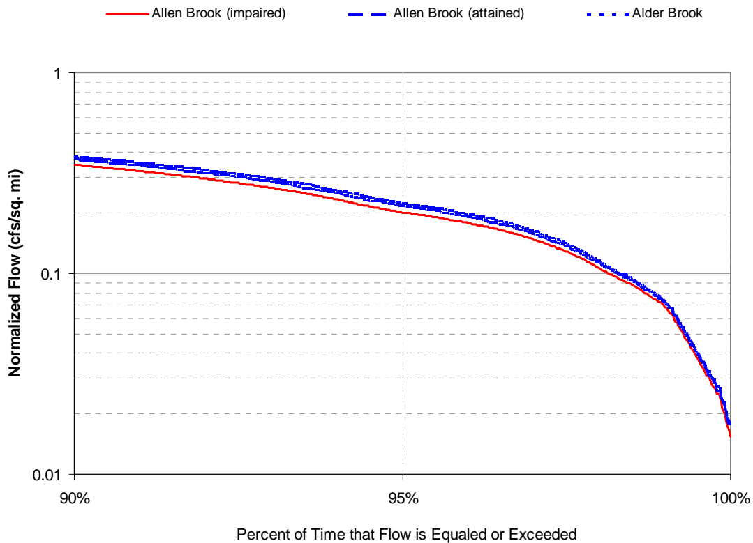
Figure 6. Low flow portion of the flow duration curves for Allen Brook and attainment streams.
